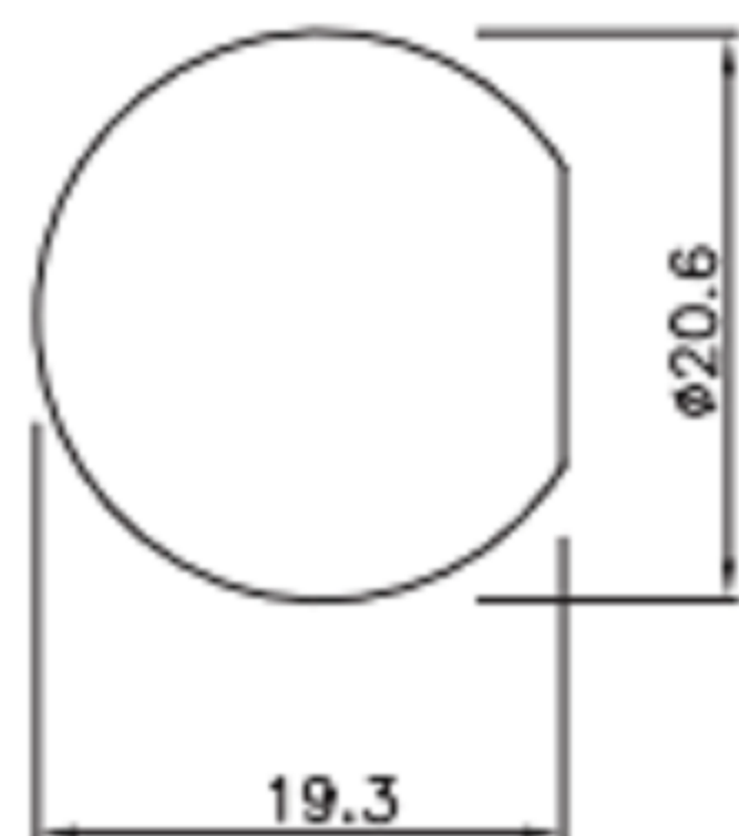
开孔尺寸 hole opening size
